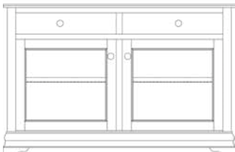
Console #3001 19"D x 55"W x 36"H
